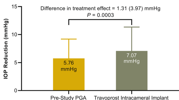
Fig. 2 IOP-lowering treatment effect and treatment effect difference. Error bars represent standard deviation. IOP intraocular pressure, PGA prostaglandin analog
